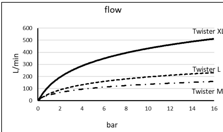
Water flow with fully opened nozzle, depending on pressure
