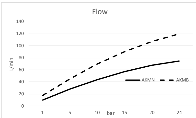
Water flow when trigger is fully squeezed, depending on pressure.
