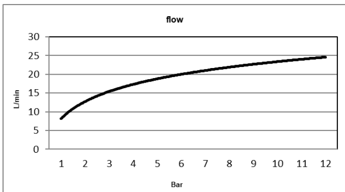
Water flow when trigger is fully squeezed, depending on pressure.
