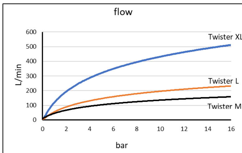
Water flow in L/min at fully opened nozzle, depending on pressure
